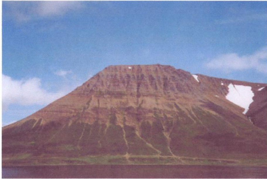
Figure 22: Overview of the westernmost sector of the Lambadalshlíð slope between the edge of the Lambadalsfjall (550 m.a.s.l.) and the Dýrafjörður fjord. The picture is taken towards the northeast.
