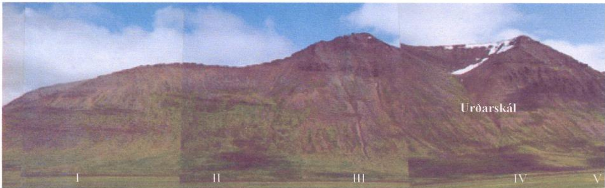
Figure 19: Overview of the Kirkjubólshjall mountain. The numbers refer to the different sectors. The picture is taken towards east-northeast.
