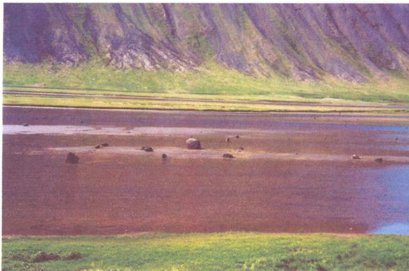
Figure 20: Boulders on flat land, in the water downhill of the fourth sector. The picture is taken towards southwest.
