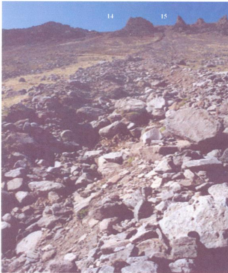
Figure 8: Erosive channel with levées downstream of the gully 15 on Eyrarhlíð.
