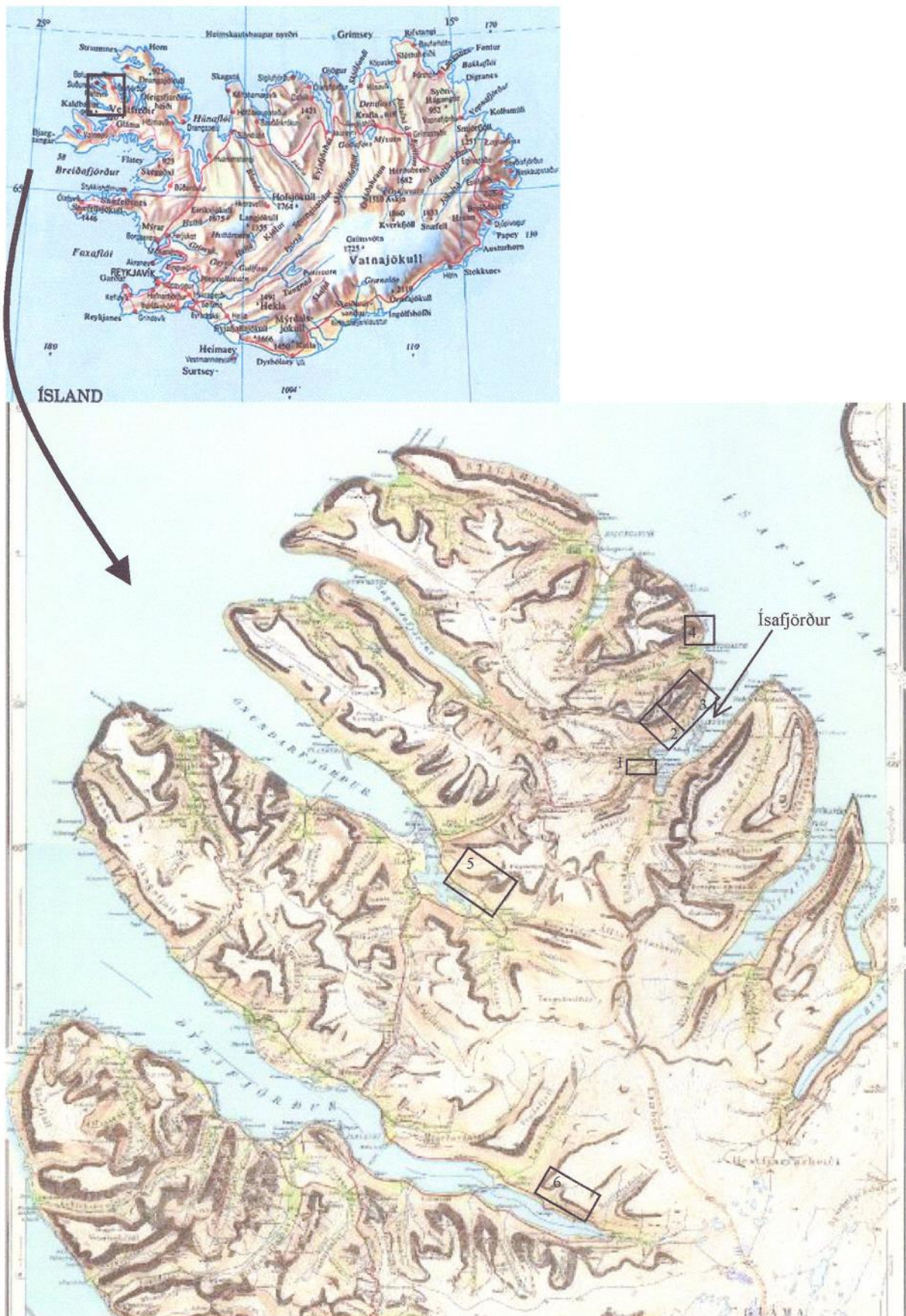
Figure 1: Locality map of the study areas in northwestern Iceland; (1) Kubbi in Skutulsfjörður; (2) inner and (3) outer parts of Eyrarhlíð in Skutulsfjörður; (4) The Hnifsdalur valley area; (5) Kirkjubólshlíð mountain in Önundarfjörður; (6) Lambadalshlíð slope in Dýrafjörður.
