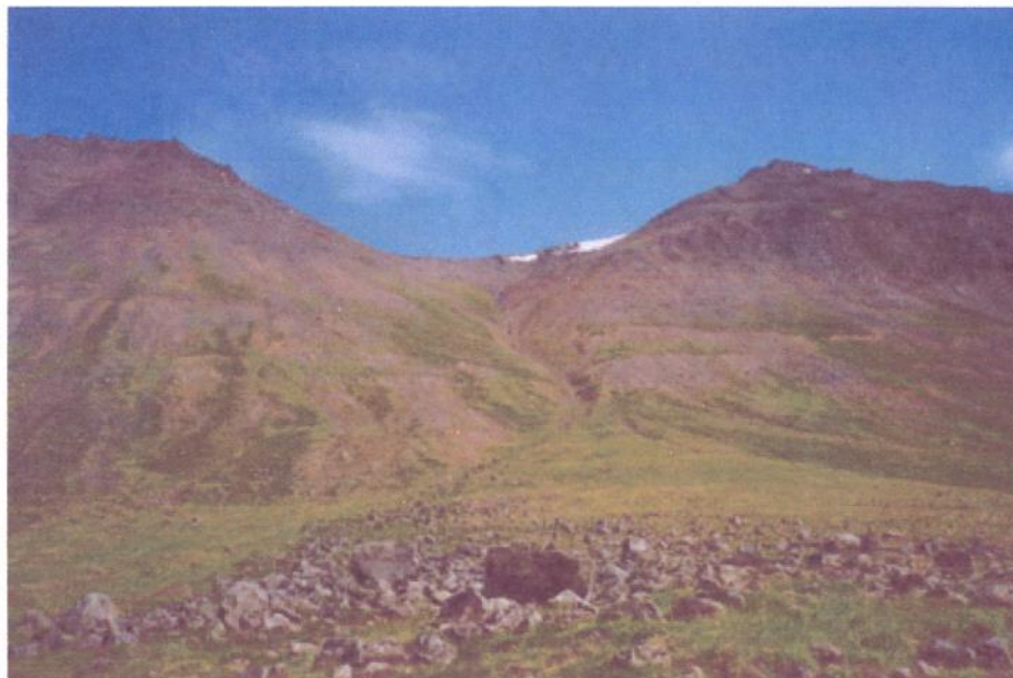
Figure 21: Urðarskál. Bowl-shaped source area and large lobe, which end progressively eastwards with vegetation whereas it ends with steeper “front” westwards with boulders. The picture is taken towards northeast.
