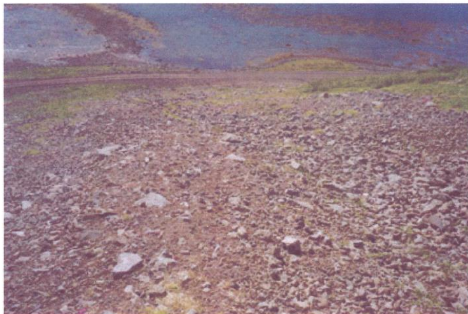
Figure 28: Detail of the low part of a track in the third sector of the Lambadalshlíð slope. Note the prograding lobes in the fjord. The picture is taken towards southeast.
